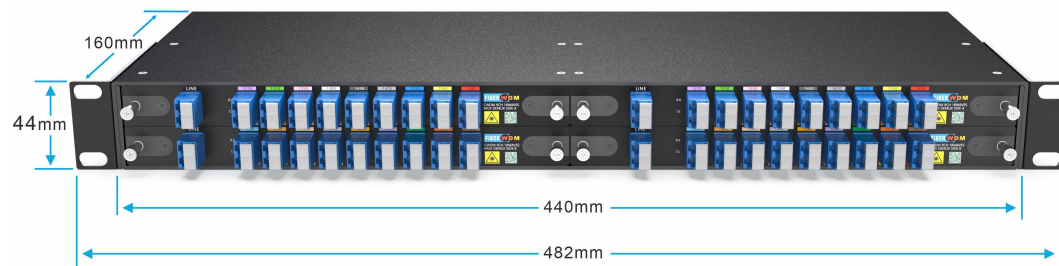
4-Slot 1U Rack for LGX BOX
