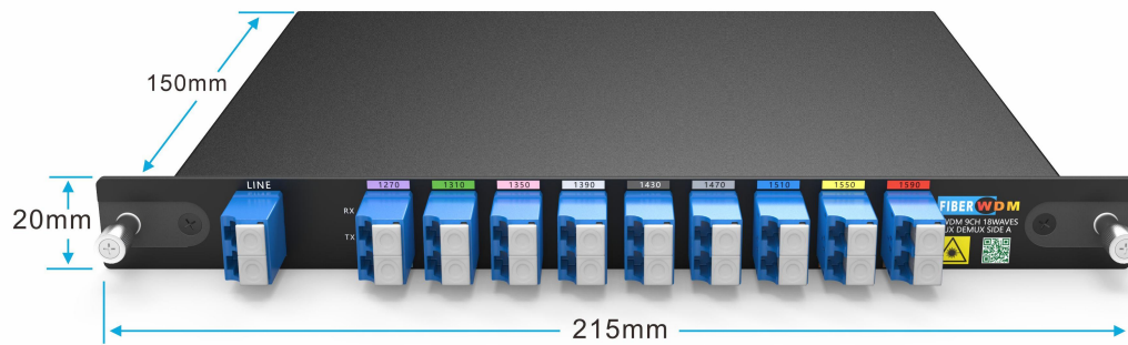
Plug-in LGX Box
