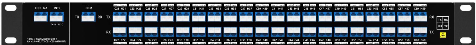
40CH 80Waves RX C21~C60 / TX H21~H60 DWDM MUX DEMUX, With INTL Port Single fiber in Side A
