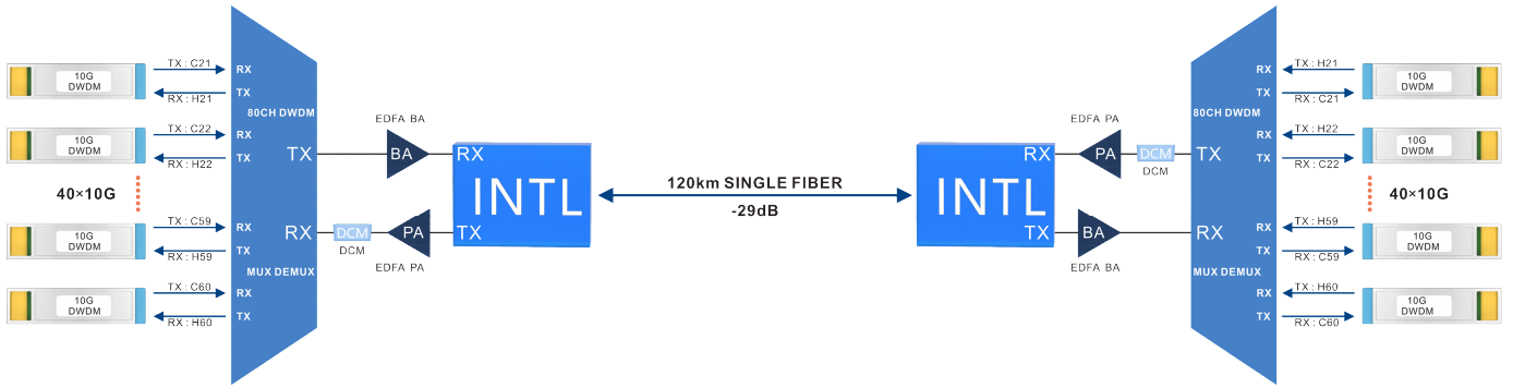
40CH DWDM MUX/ DEMUX Single fiber BIDI transmission
